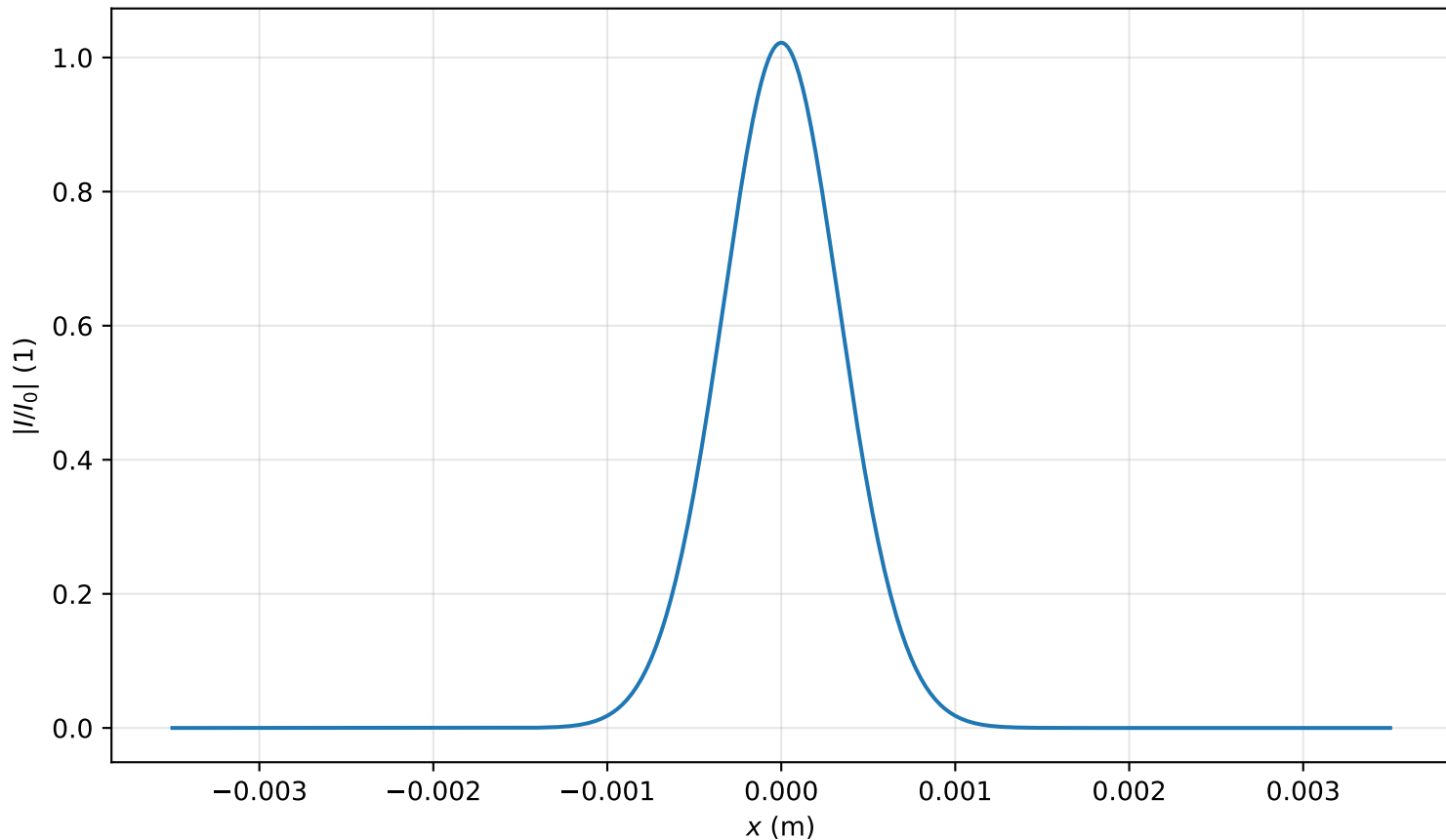
Intensity profile I(x, y = 0, z = 0.318m)/I_0 , P_{in}=0.5P_{cr} , artificial time
